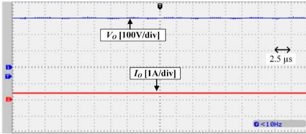
Fig. 11. Output voltage and current waveforms of the modified cascaded Z-source high step-up boost converter.
