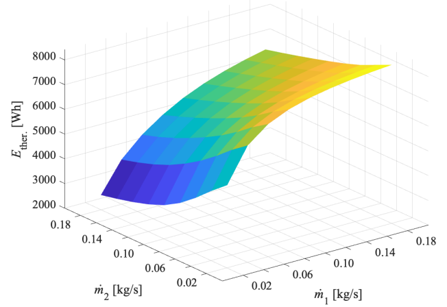
Fig. 8. Daily production of thermal energy E_{ther.} of the PV/T system as a function of the change in mass flow of the PV/T modules \dot{m}_1 and the mass flow of TEST \dot{m}_2 .
