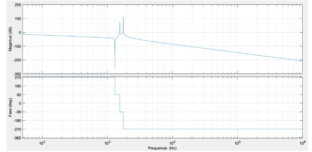
Fig. 4. Bode plot of the function F_v(s) .
