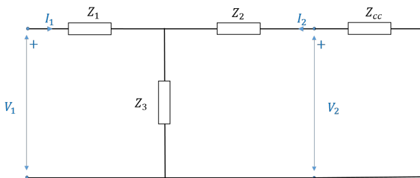
Fig. 3. Equivalent circuit of the filter considering grid effects.
