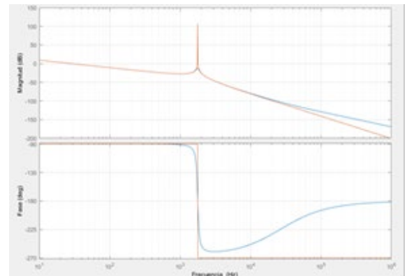
Fig. 2. Bode plot of the function G_v(s) with R_3 = 0 \Omega (in red) and with attenuation R_3 = 1 \Omega (in blue).
