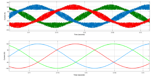
Fig. 6. Current waveforms of the inverter-side and the grid-side of the SiC inverter.
