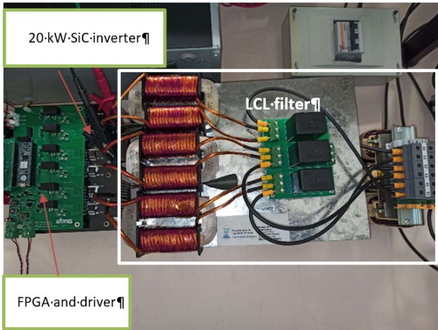
Fig. 5. 20 kW SiC inverter and the LCL filter prototype.
