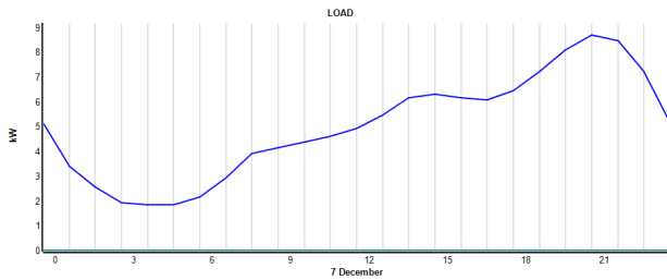
Fig. 2. Load consumption of the day December 7 th .
