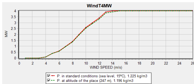
Fig. 2. Wind turbine output power curve (MW) vs wind speed (m/s).
