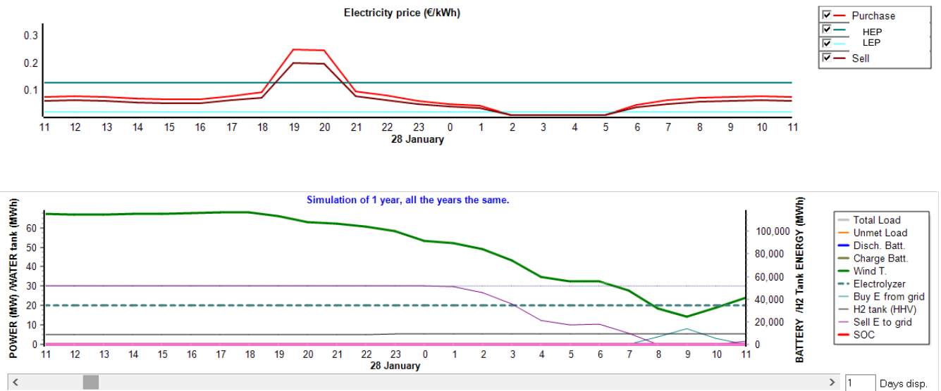
Fig. 8. Simulation of the system, shown January end of day 27 th – first of day 28 th . MHOGA software
