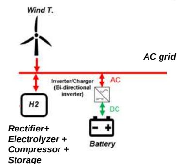
Fig. 1. Hydrogen generating system powered by wind turbines + grid + battery.
