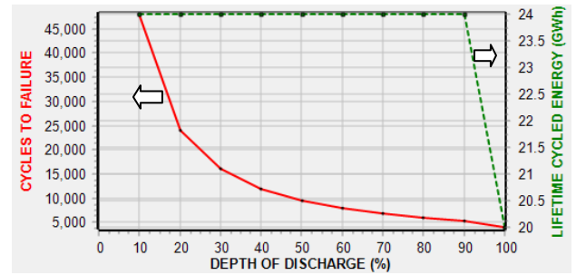
Fig. 4. Cycles to failure (red, left axis) and lifetime cycled energy (GWh, green, dash, right axis) vs depth of discharge, DOD (%). 5 MWh battery unit.
