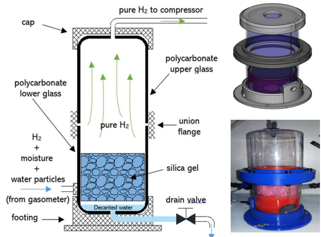
Fig. 7. Desiccator.
