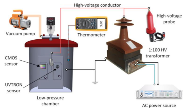
Fig. 2. Sketch of the experimental setup.
