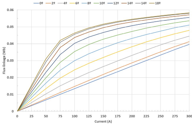
Fig.11. Magnetization curves SSSRM AI
