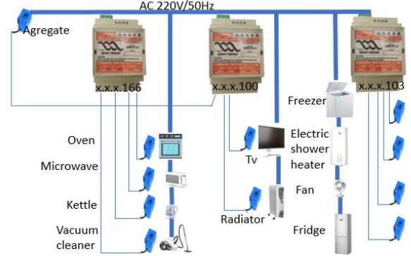
Fig. 1. oZm's connections with the applications.
