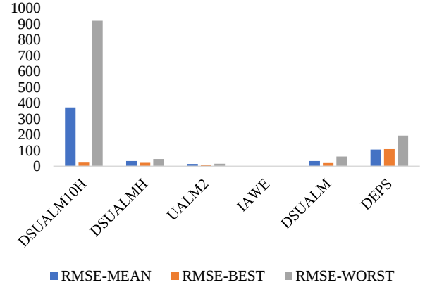
Fig. 9. RMSE metric comparison using the mean, best or worst value.
