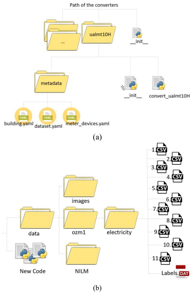
Fig. 3. (a) Data file structure. (b) Metadata file structure.
