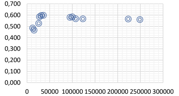
Fig. 5. Relationship between the number of samples and F1-score.
