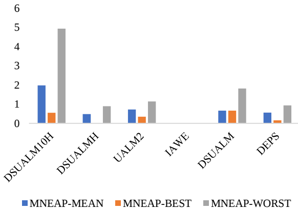
Fig. 8. MNEAP metric comparison using the mean, best or worst value.
