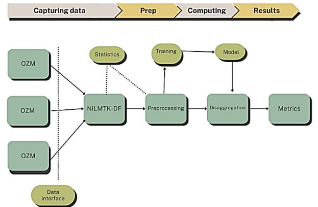
Fig. 2. NILMTK flow diagram.
