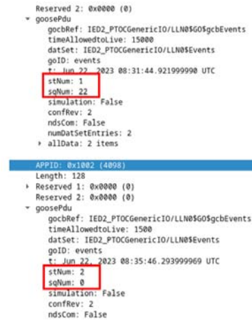
Fig.13.Identification of operation time with Wireshark
