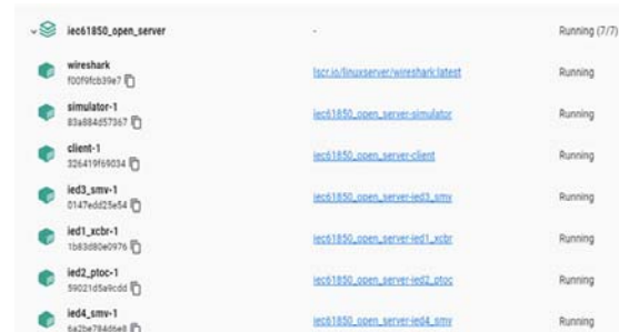
Fig.7. Docker containers
