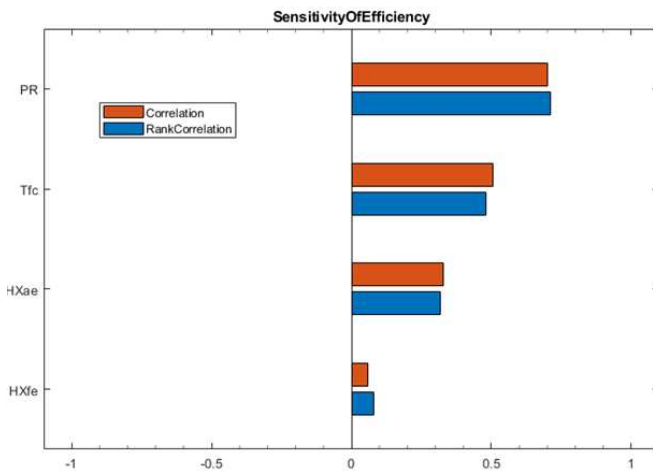
Fig. 2. Tornado plot from sensitivity analysis of steady state simulation results.
