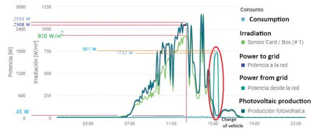
Fig. 10. Curves of relevant variables observed during the charging process of the electric vehicle.
