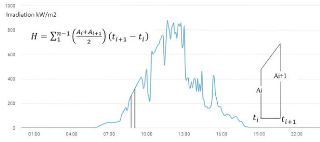
Fig. 1. Irradiation ( \text{W/m}^2 ) in the installation place.
