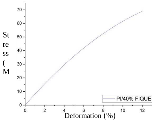
Fig. 1. Tensile stress vs strain diagram, 40% Fique biocomposite
