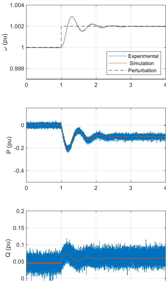
Figure 7. Simulation and experimental data under a frequency perturbation of 0.002 pu
