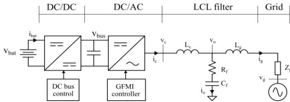
Figure 1. Schematic of the electrical test bench.
