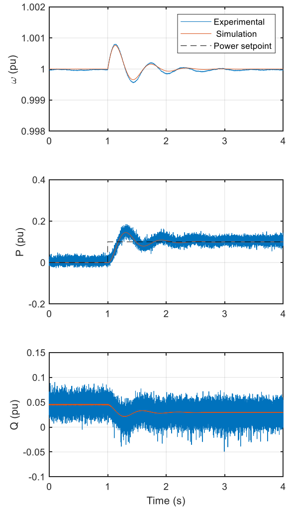
Figure 6. Simulation and experimental data under a power setpoint step of 0.1 pu
