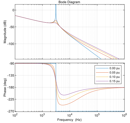
Figure 3. LCL filter response under different damping resistors.
