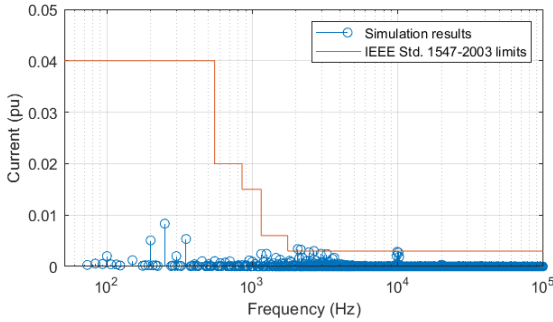
Figure 2. Grid current harmonic spectrum for selected L_g .
