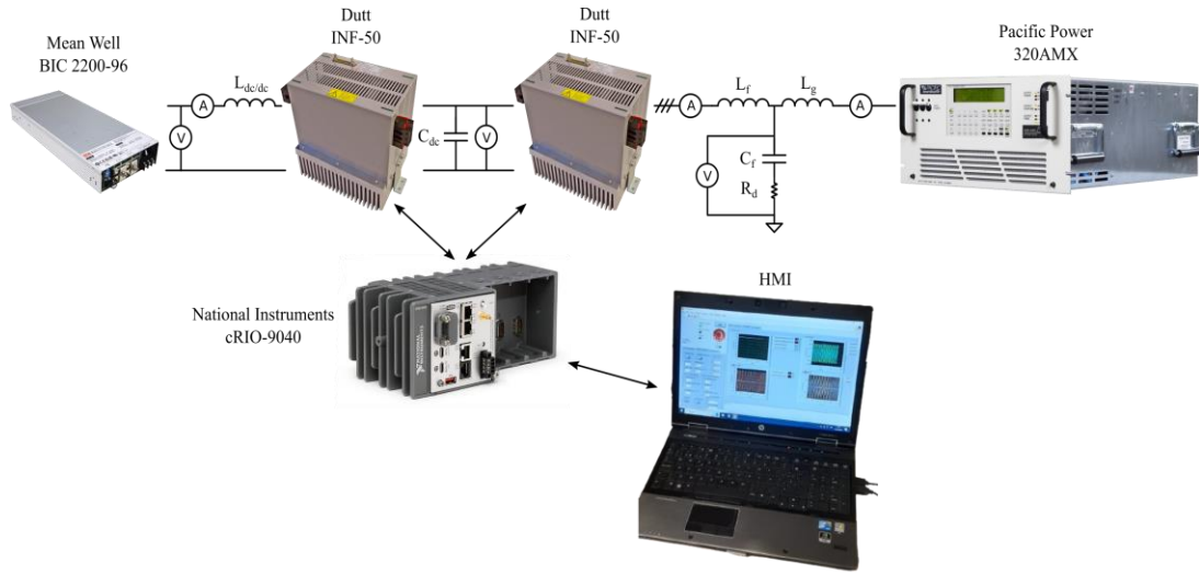
Figure 5. Schematic of the test bench for validating control strategies.
