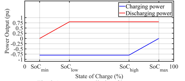
Fig. 2 Output power limits of battery.
