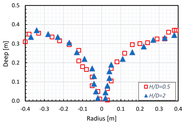
Figure 11. Vortex profile for L_c/D = 0.7 , w_2/D = 0.4
