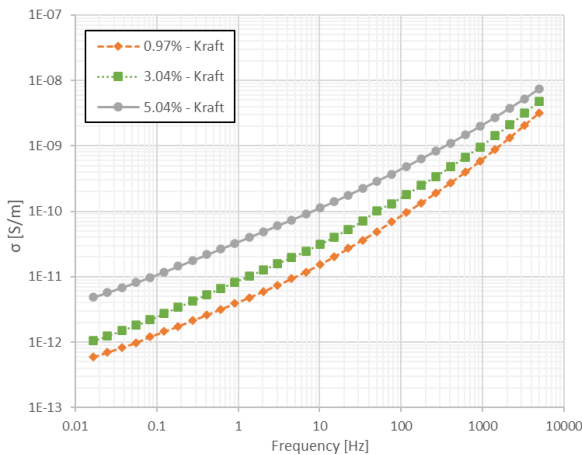
Fig. 13. \sigma of Kraft paper samples with different m.c.
