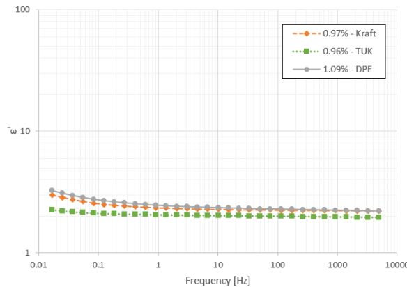
Fig. 3. Comparative of \epsilon' of samples with 1% m. c.
