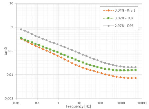
Fig. 5. Comparative of \tan \delta of samples with 3% m. c.
