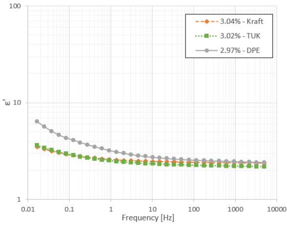
Fig. 6. Comparative of \epsilon' of samples with 3% m. c.
