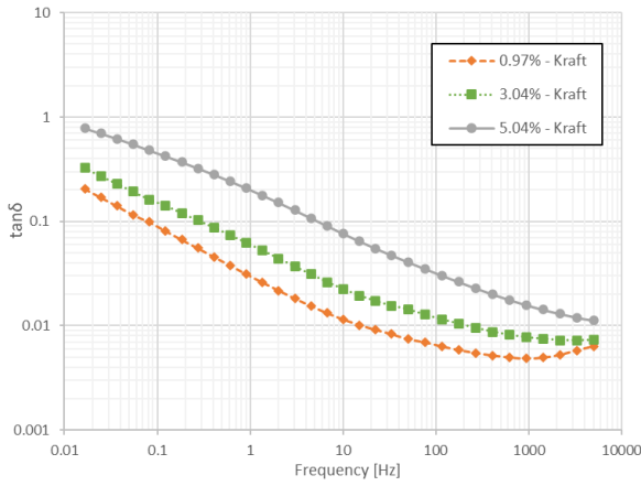
Fig. 11. \tan \delta of Kraft paper samples with different m.c.
