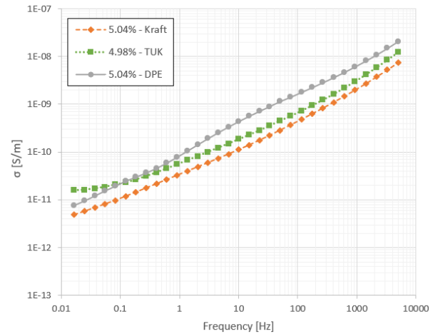
Fig. 10. Comparative of \sigma of samples with 5% m. c.
