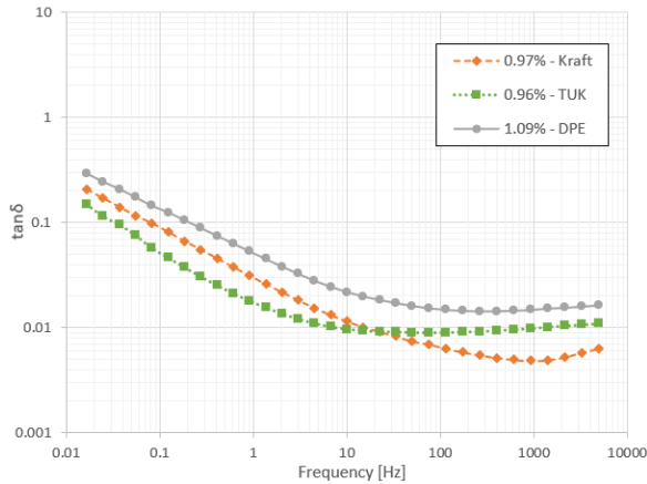
Fig. 2. Comparative of \tan \delta of samples with 1% m. c.
