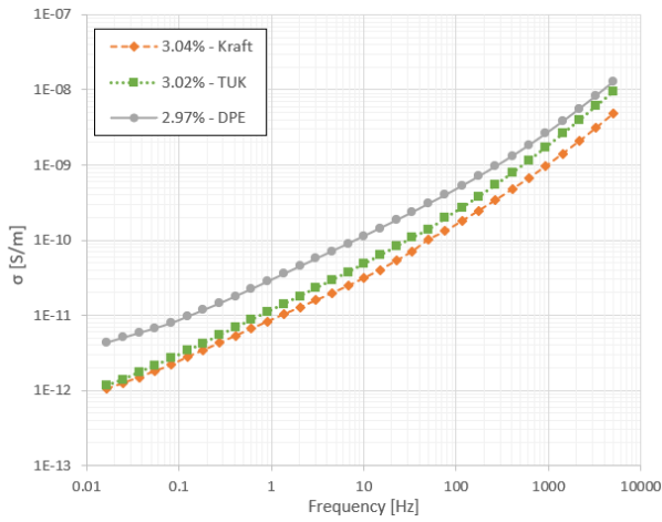
Fig. 7. Comparative of \sigma of samples with 3% m. c.
