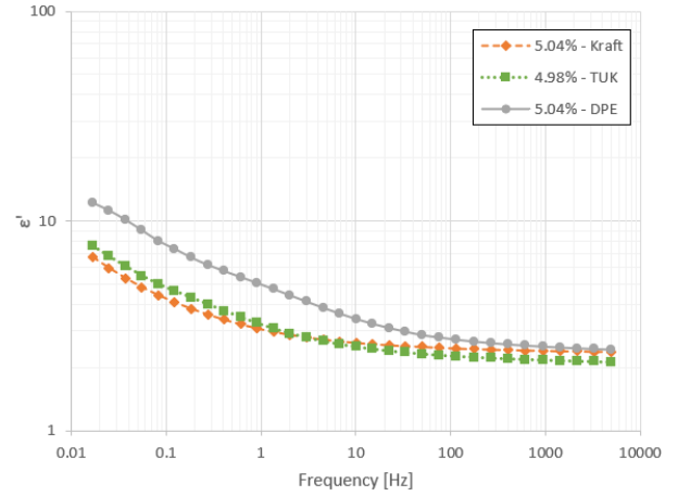
Fig. 9. Comparative of \epsilon' of samples with 5% m. c.
