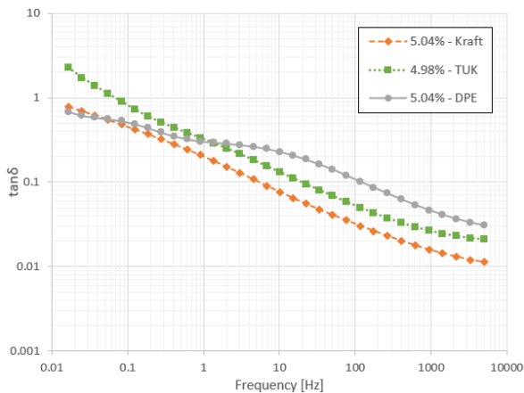
Fig. 8. Comparative of \tan \delta of samples with 5% m. c.
