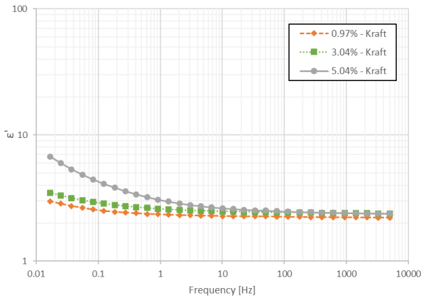
Fig. 12. \epsilon' of Kraft paper samples with different m.c..
