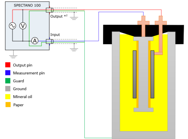
Fig. 1. Test cell connection diagram
