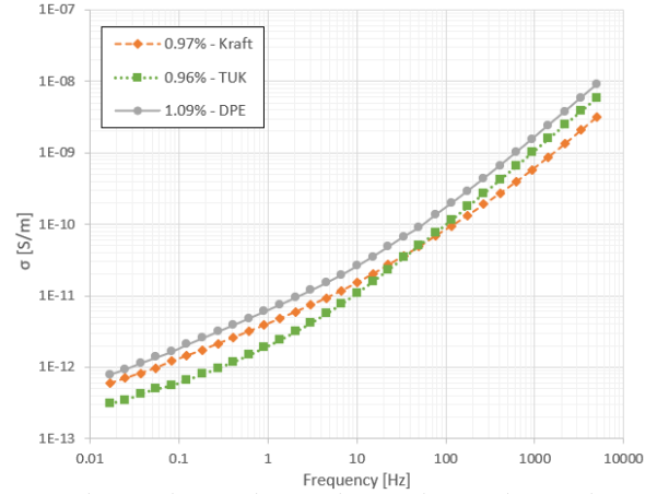
Fig. 4. Comparative of \sigma of samples with 1% m. c.
