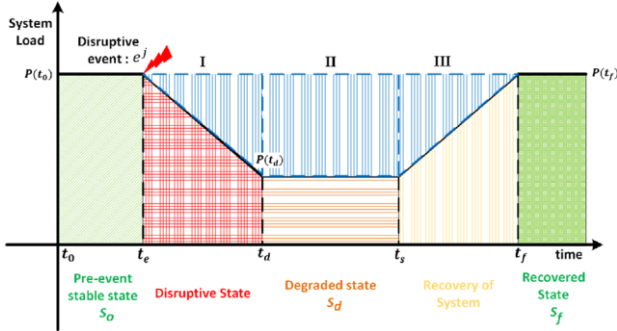
Fig. 1. Resilience curve representing network operation states.
