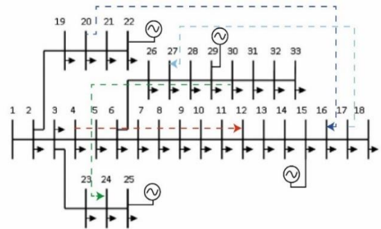
Fig 2. IEEE 33 bus modified system.
