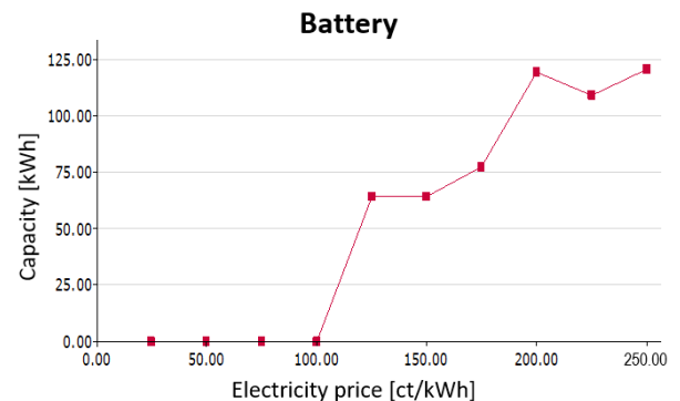
Fig. 9. Battery sensitivity analysis
