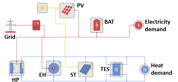
Fig. 4. Configuration of cases 1 and 2
