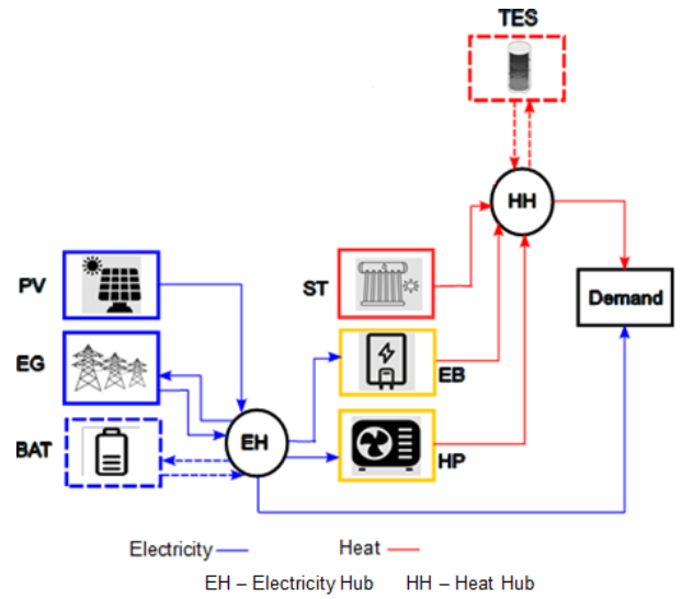
Fig. 3. Overview of decarbonisation energy concepts (adapted from [6])
