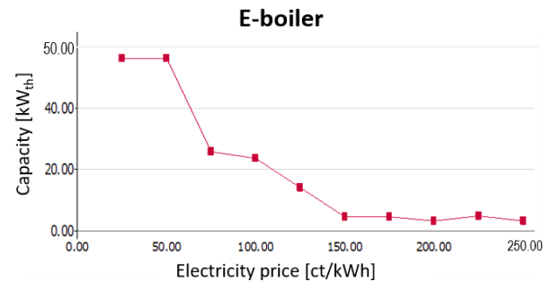
Fig. 8. EB sensitivity analysis
