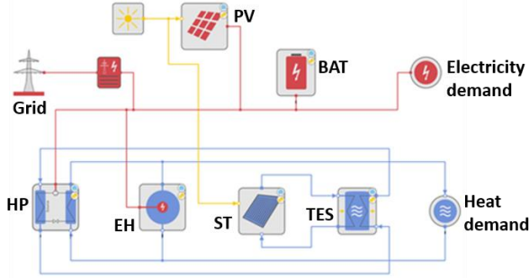
Fig. 6. Configuration of case 4
