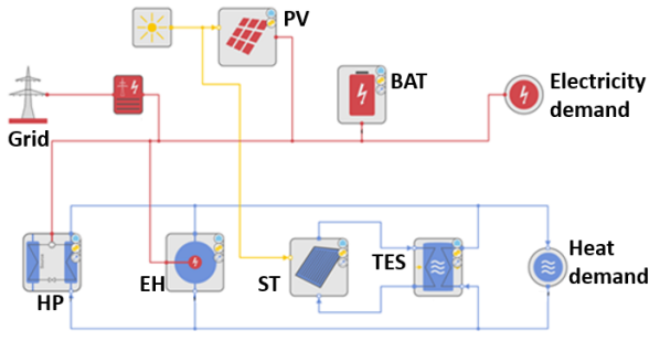
Fig. 5. Configuration of case 3
