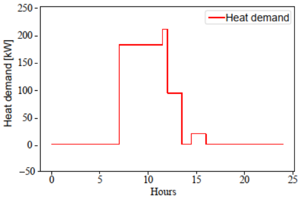
Fig. 2. Daily heat demand for operation with steam
