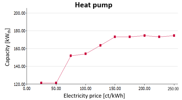
Fig. 7. HP sensitivity analysis
