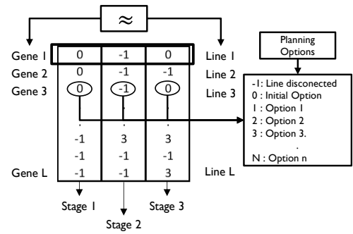
Fig. 3. Chromosome Encoding.
