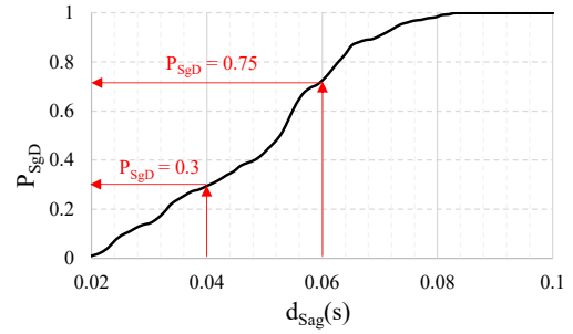
Fig. 1. Cumulative distribution function for voltage sag duration. Adapted from [7].
