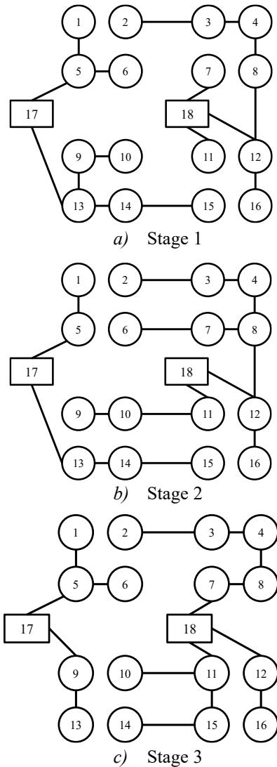
Fig. 6. Topology of the best result.
