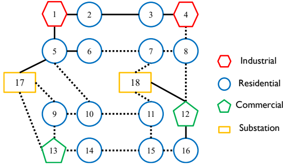
Fig. 4. Network of 18 Bus Adapted from [8]
