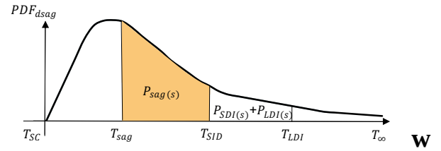
Fig. 2. Time interval for the probability of transients, sags, SDI, and LDI
