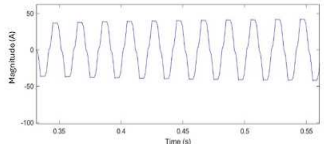
Fig.6. Current waveform on busbar 22
