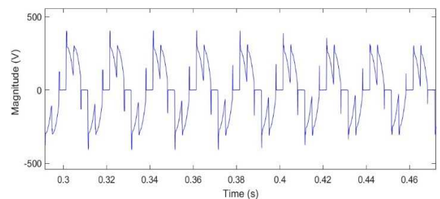
Fig.7. Voltage waveform on busbar 22
