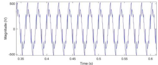
Fig.14. Voltage waveform on busbar 2
