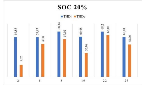
Fig.5. THDi and THDv for a SOC of 20%
