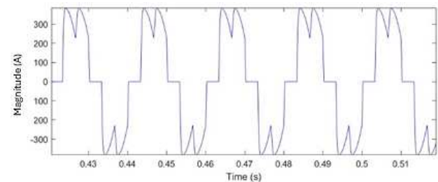
Fig.13. Current waveform on busbar 2
