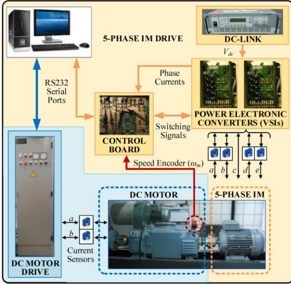
Fig. 2. Diagram and photographs of the laboratory setup used in the experiments.
