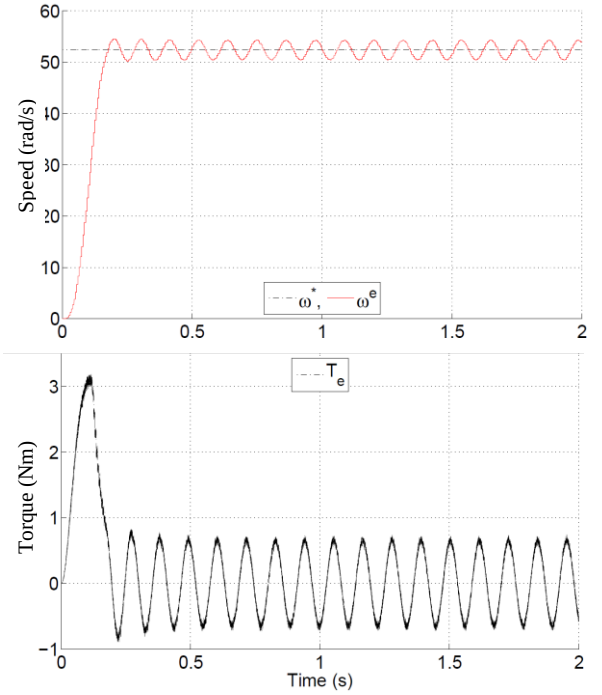
Fig. 3. Trajectories of speed (top) and torque (bottom) for a step test using tuning T1.
