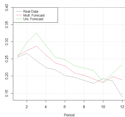
Fig. 6. Out-of-sample forecast of the variation of Installed Capacity in megawatts (MW) in Brazil using the two RNA arrangements compared in this research (see equation 1 and 2). Source: own elaboration
