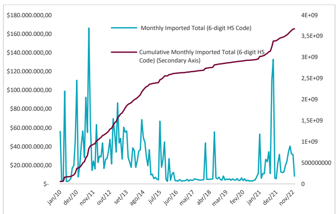
Fig. 1. Imports of components for wind energy production from 2010 to 2022, monthly data
