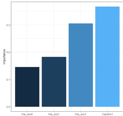
Fig. 4. Relative Importance of Input Variables in Neural Networks Using Garson's Algorithm Source: own elaboration
