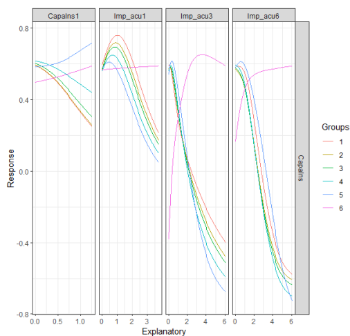
Fig. 5. Sensitivity Analysis Using Lek Profile Method, where in the analysis of each predictor variable the others were kept at their minimum values, 1st quartile, median, 3rd quartile, and maximums (Groups from 1 to 6, respectively). Source: own elaboration
