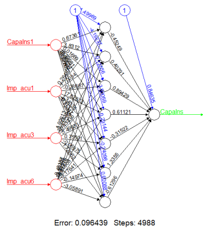
Fig. 3. Artificial Neural Network – Configuration ( net_{1t} ) (Equation 1) Source: own elaboration
