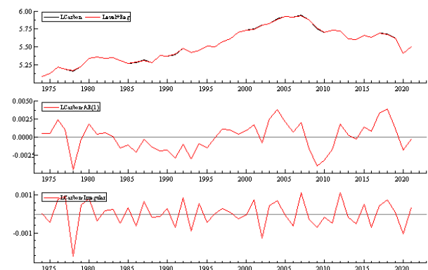
Fig.2. Model fitting
