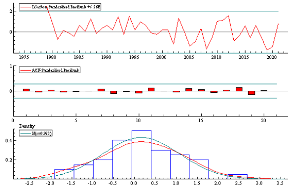
Fig. 3. Model residuals
