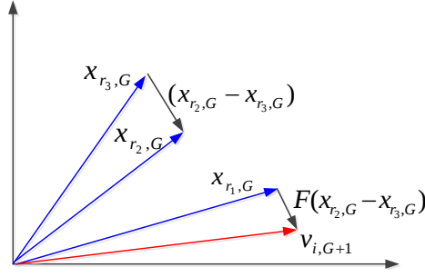
Fig. 2. Graphic representation of the mutation process of the differential evolution method.
