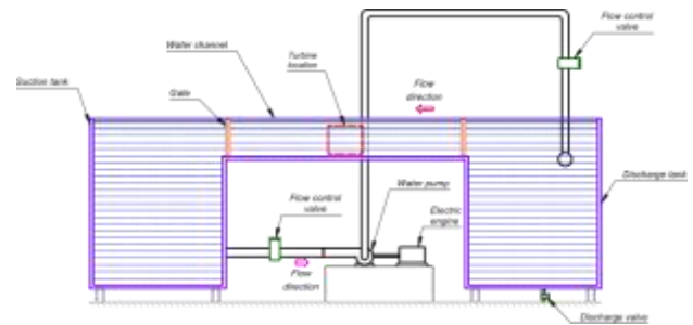
Fig 1. General configuration design of the experimental installation
