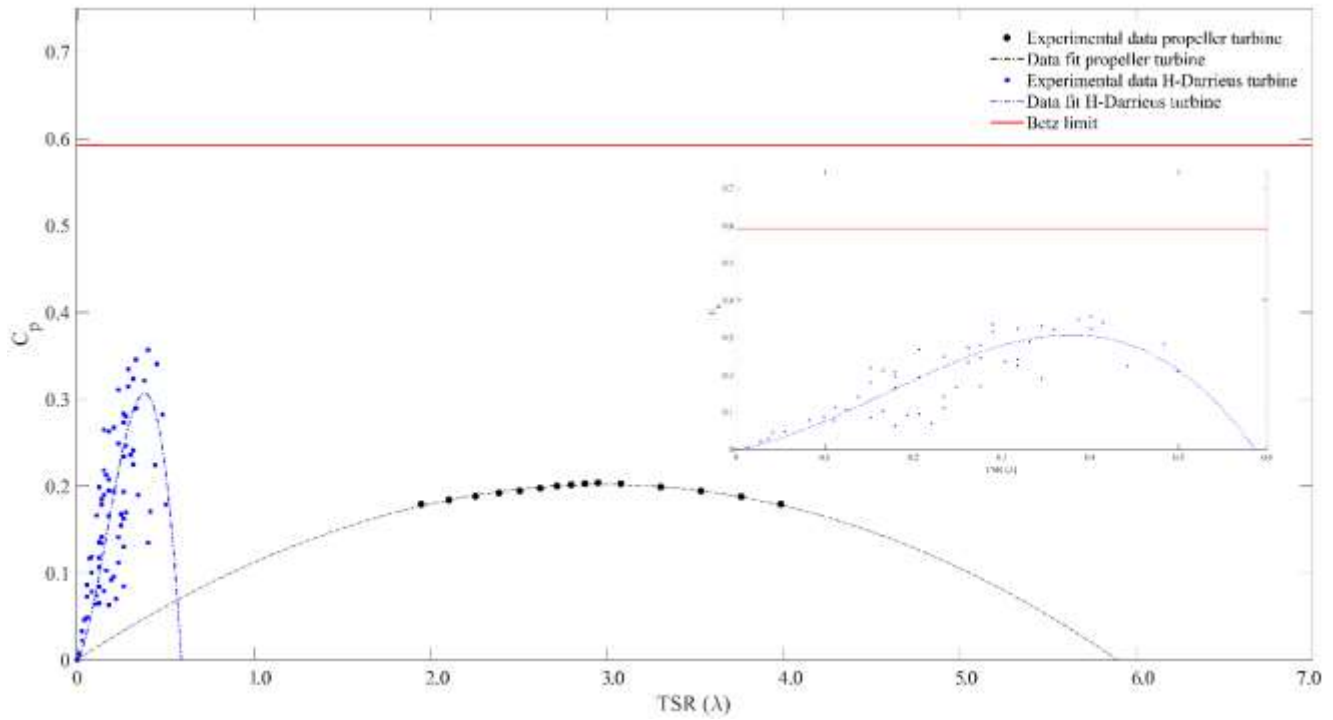
Fig. 6. Power coefficient ( C_p ) vs. tip speed ratio (TSR) values
