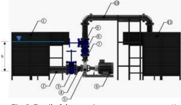
Fig. 2. Detail of the pumping system components. 1) Suction tank, 2) suction pipe, 3) gate valve, 4) eccentric reducer, 5) pump, 6) motor, 7) concentric reducer, 8) check valve, 9) gate valve, 10) discharge pipe, 11) Discharge tank
