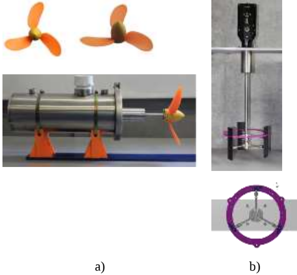
Fig. 5. a) Propeller hydrokinetic turbine, b) H-Darrieus hydrokinetic turbine
