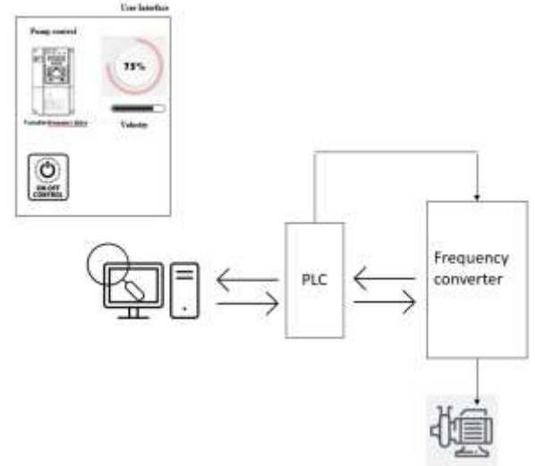
Fig. 3. Control system interface for the pumping system
