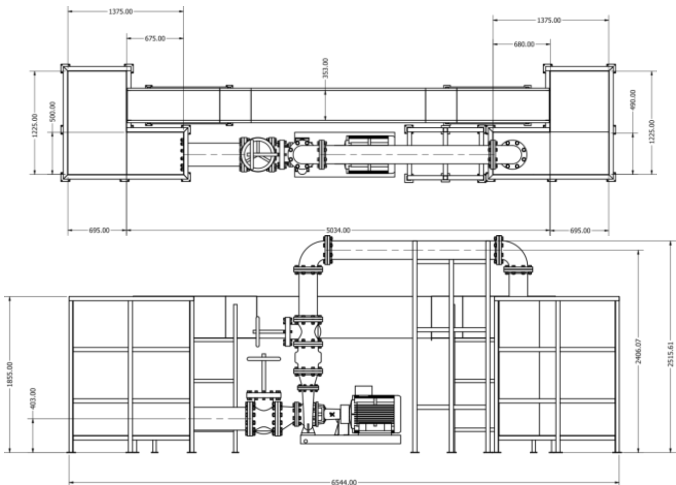
Fig. 4. Overall dimensions of the experimental installation. Measurements are expressed in mm
