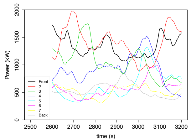
Figure 4. Power output from turbines in column C during final 600 s of computer simulation for the wind direction of 207^\circ .
