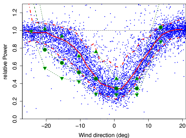
Figure 5. Relative power deficit of turbine D07 in second row compared to front turbine D08. Blue dots: SCADA data; red line: median over 2° window, red dashed lines: range covering 75% of measurements; green circles: median of CFD results, green triangles: range covering 75% of results. Direction 0° denotes turbine row fully aligned with wind.
