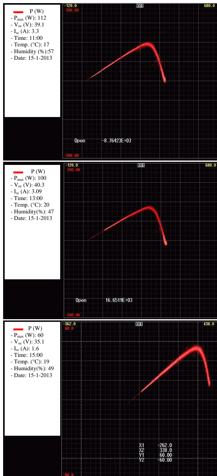
Fig. 8. P-V curves for poly-crystalline 120W-PV at different times on January 15, 2013.
