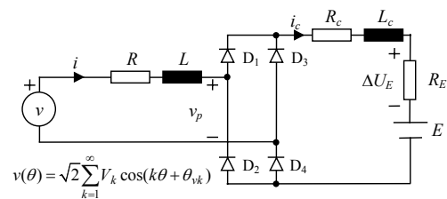
Fig. 1. Equivalent circuit of EV battery chargers.
