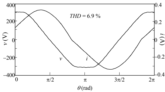
Fig. 4. Measured current waveforms of CCM2.
