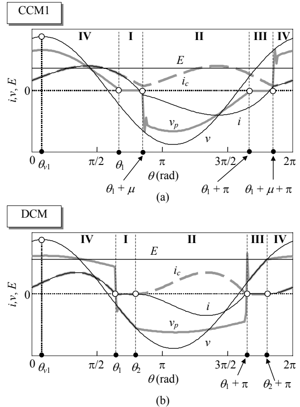
Fig. 3. EV battery charger modeling.
