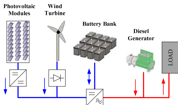
Fig. 3. Mixed DC- and AC-coupled concept
