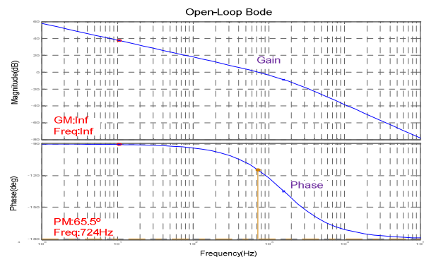
Fig. 4. Open-Loop Bode of GOL(s).
