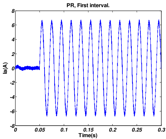
Fig. 23. Phase a current wave form in the first interval of simulation with PR control.
