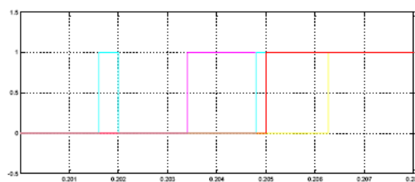
Fig. 2. Detection time for the different methods: Fourier (yellow), Matrix (pink), peak value (blue), RMS value (red).
