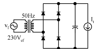
Fig. 1 Configuration of a traditional AC-DC power supply.
