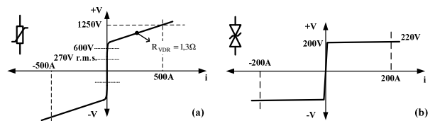
Fig. 10 Voltage and current characteristic curves: (a) 250Vrms VDR; (b) 200V bipolar Zener diode.
