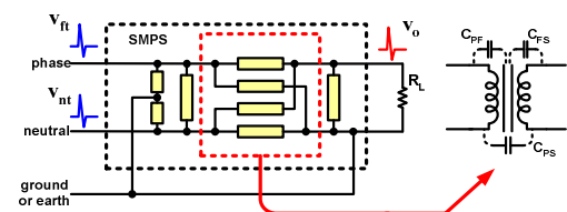
Fig. 12 High frequency impedance model.
