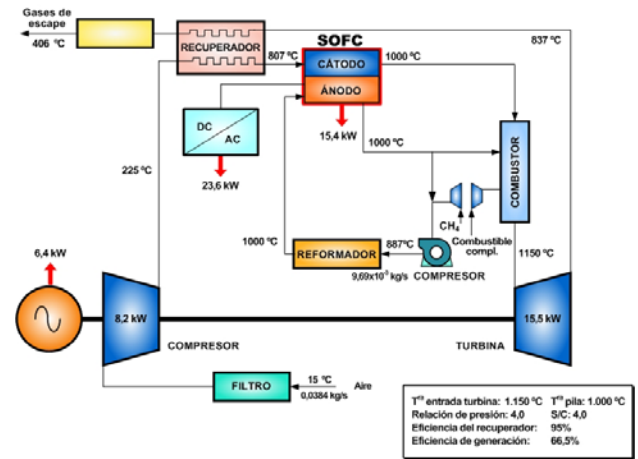
Fig.4. Scheme of SOFC – Gas Micro Turbine hybrid system
