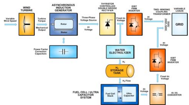
Fig.6. Wind Turbine – FC – UC hybrid system
