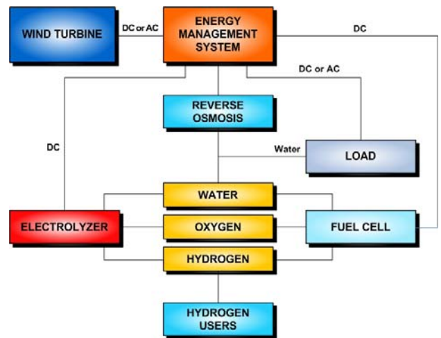
Fig 7. Wind Turbine - FC hybrid system
