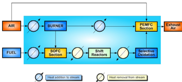
Fig.3. Scheme of SOFC – PEMFC hybrid power system
