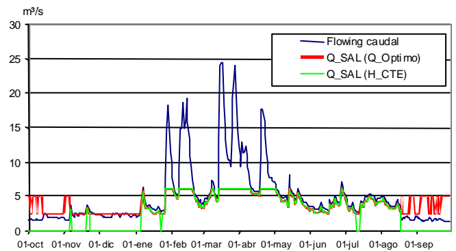
Fig. 10. Working flows ( Q_{SAL} )
