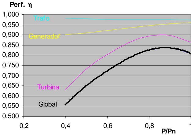
Fig. 8. Performance curves of the machines and global
