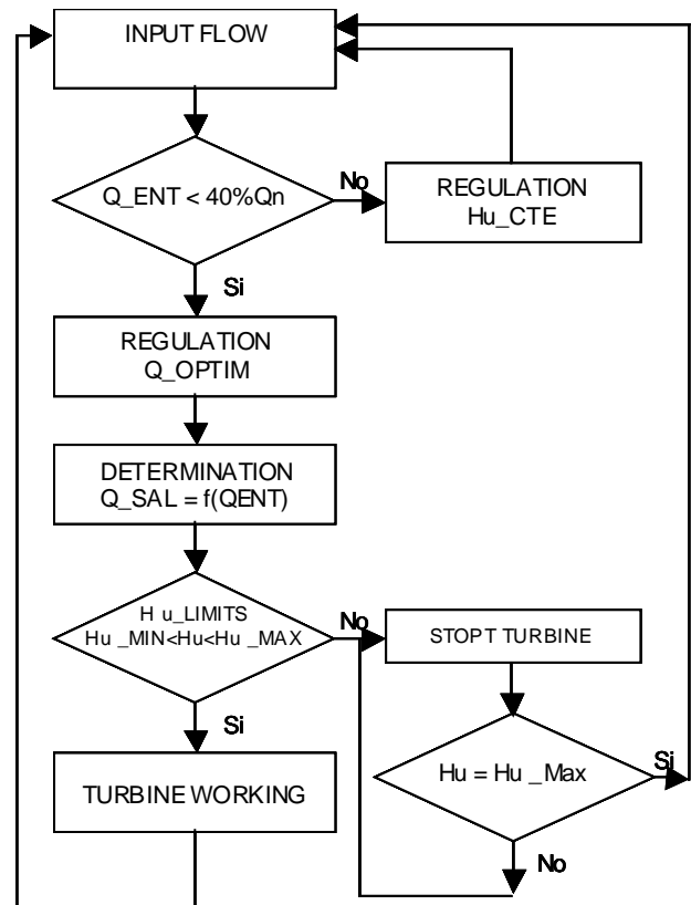
Fig. 7. Working sequence
