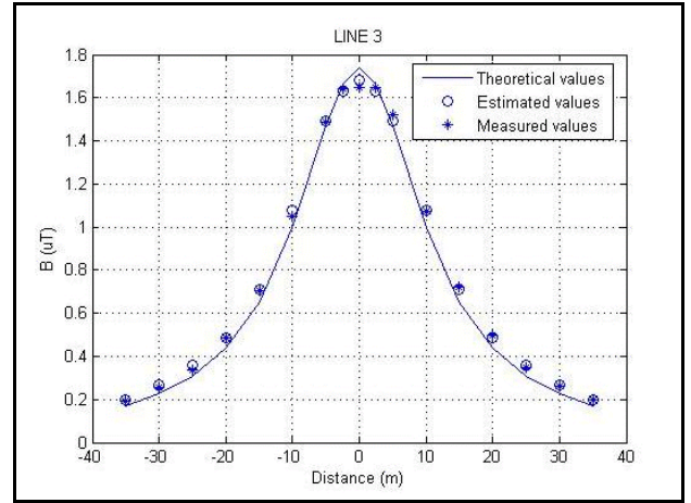
Fig 10. Line 3 (comparison of values)
