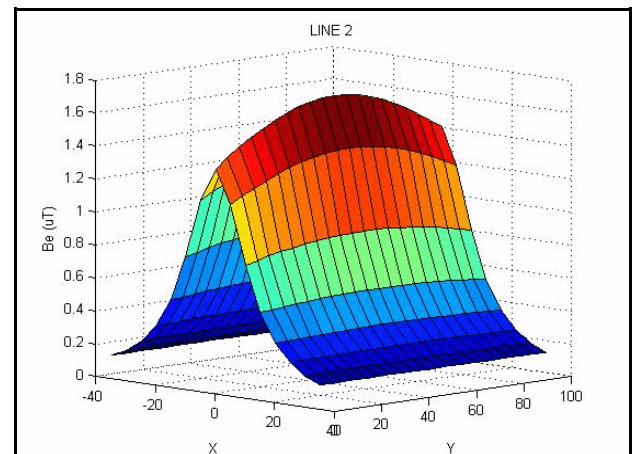
Fig 8. Line 2 (longitudinal section)
