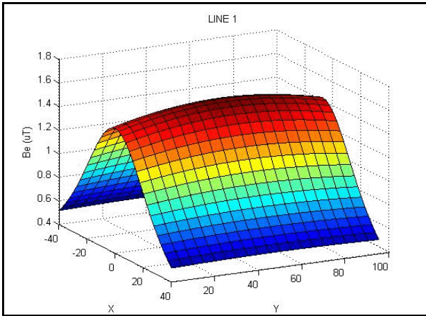
Fig 4. Line 1 (longitudinal section)
