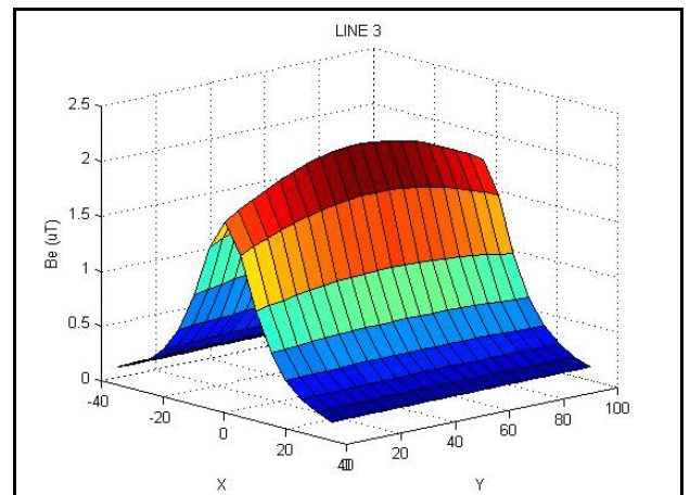
Fig 12. Line 3 (longitudinal section)
