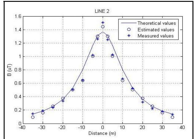
Fig 6. Line 2 (comparison of values)
