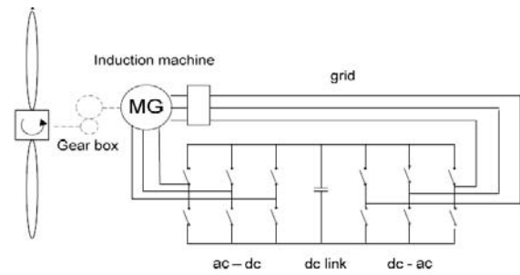
Fig. 13 Limited range, variable wind energy conversion system. (Courtesy of [7])
