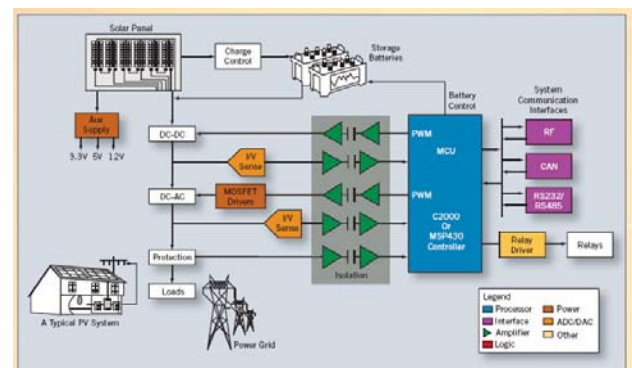
Fig. 19. Conventional power converter architecture. (Courtesy of [11])
