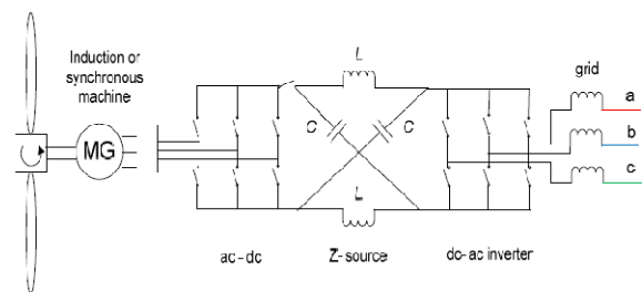
Fig. 15. Z-source based variable speed wind energy conversion system. (Courtesy of [7])
