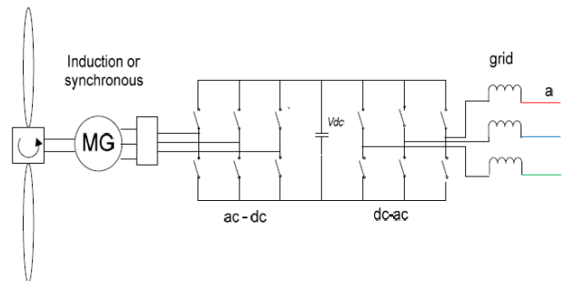
Fig. 14. Fully variable wind energy conversion system. (Courtesy of [7])
