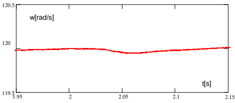
Fig 20. Speed of the motor during the sag event under the effect of the vector control system
