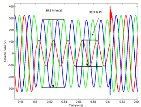
Fig. 9. Phase voltages during a type D_R sag
