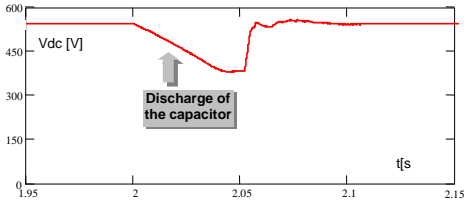
Fig 19. Decrease of the DC bus voltage under sag
