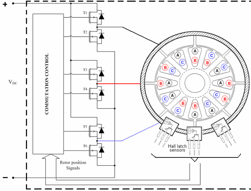
Fig. 2. Block diagram of an outside-spin brushless D.C. motor drive
