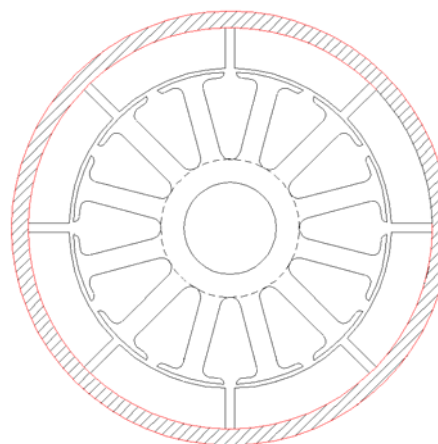
Fig. 1. Cross section of an eight-pole outside-spin brushless D.C. motor
