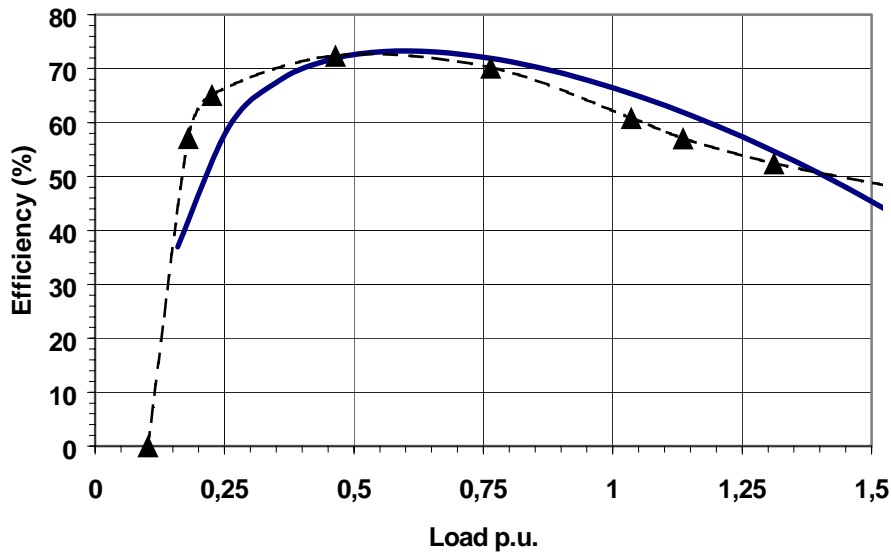
Fig. 4. Efficiency (%) versus load (p.u.). The straight line was obtained using the expressions proposed, and discontinuous line shows the experimental results
