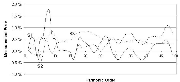
Fig. 3. Measurement error of solid state energy meters under active harmonic energy.
