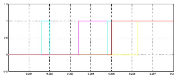
Fig. 2. Detection time for the different methods: Fourier (yellow), Matrix (pink), peak value (blue), RMS value (red).
