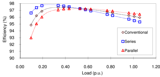
Fig. 2. Comparison of efficiency of 1kVA conventional and switchable transformer[2].
