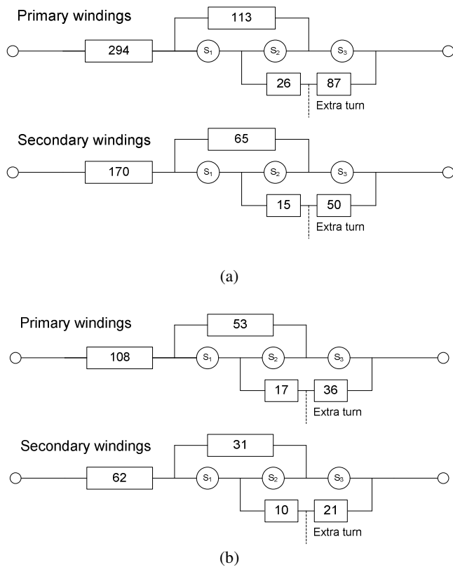
Fig. 9. The tapings of windings of the three-phase switchable transformers: (a) 3 kVA built in 2002 (b) 10 kVA built in 2003.
