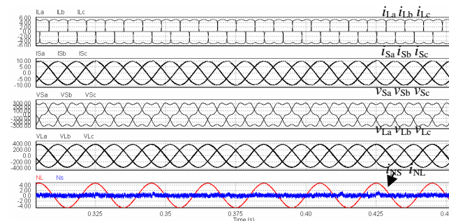
Fig. 6. Load-mains currents and voltage waveforms.
