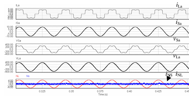
Fig. 7. Load-mains current and voltage waveforms in phase "a".
