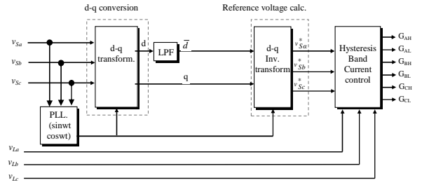
Fig. 3. Series active power filter control block diagram.
