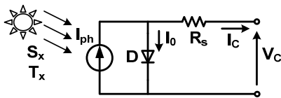
Fig. 3. One diode equivalent parameters PV model.
