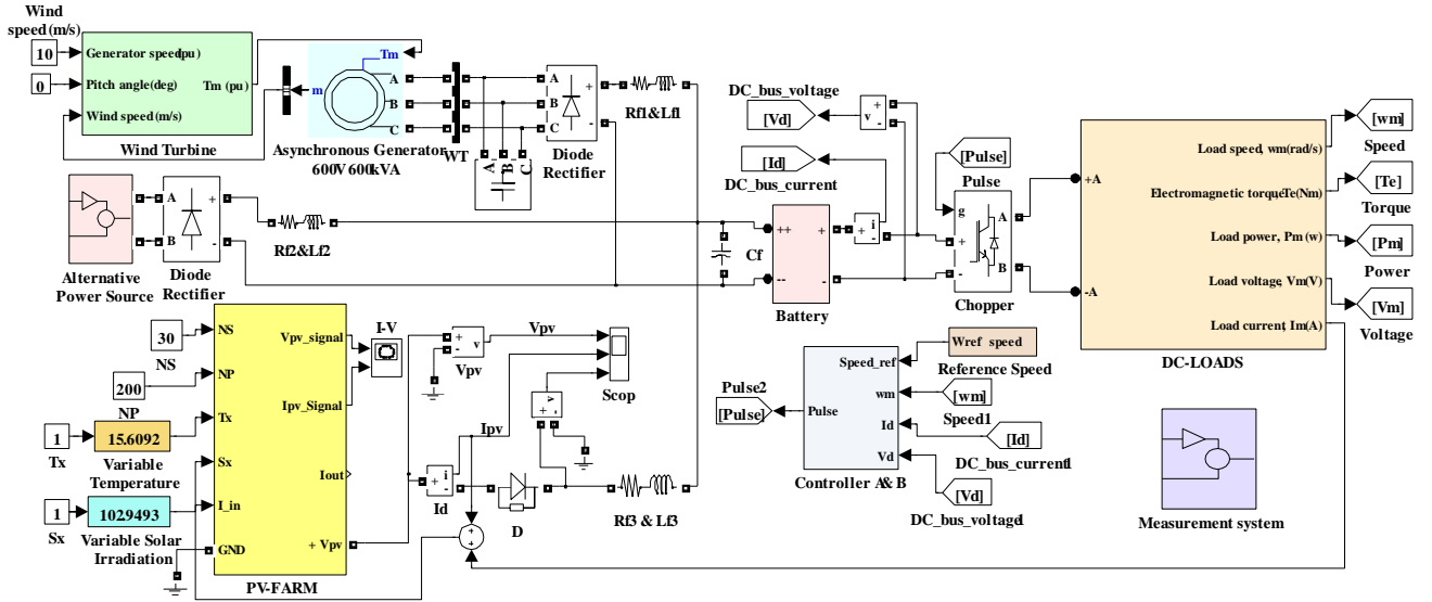
Fig. 6. The proposed hybrid renewable energy system Simulink block diagram.
