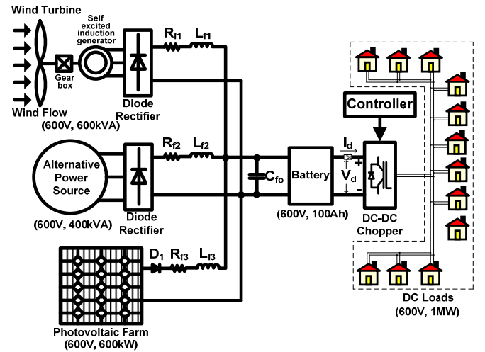
Fig. 1. Proposed grid-connected Wind/PV power generation system.
