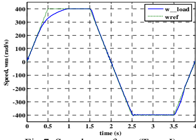
Fig. 7. Speed waveform (Type I)
