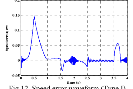
Fig. 12. Speed error waveform (Type I)
