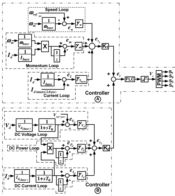
Fig. 4. Six-loop dynamic error driven fuzzy logic controller.
