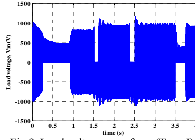
Fig. 9. Load voltage waveform (Type I)
