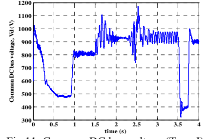
Fig. 11. Common DC bus voltage (Type I)
