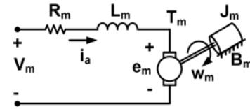
Fig 2. The equivalent circuit of a dc motor
