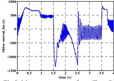
Fig. 8. Motor current waveform (Type I)
