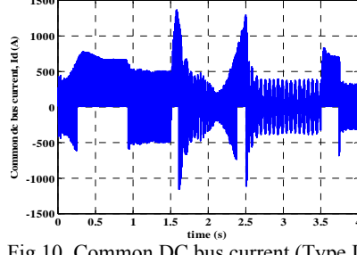
Fig. 10. Common DC bus current (Type I)
