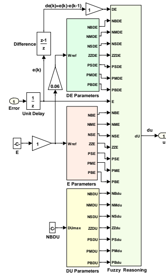
Fig. 5. Details of the fuzzy reasoning block.
