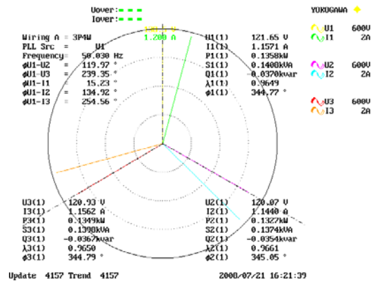
Fig.11 Phasors of source phase voltages and currents
