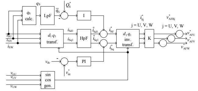
Fig.8 Control strategy of HPH
