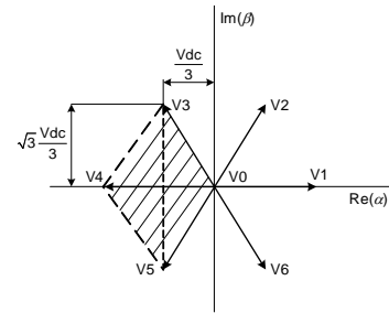
Fig.2 Voltage space-vectors in proposed converter
